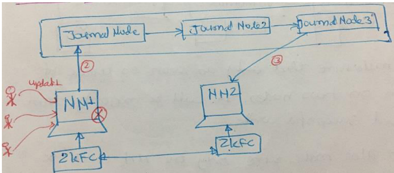
Hadoop NameNode: Active and StandBy namenode co-ordination
