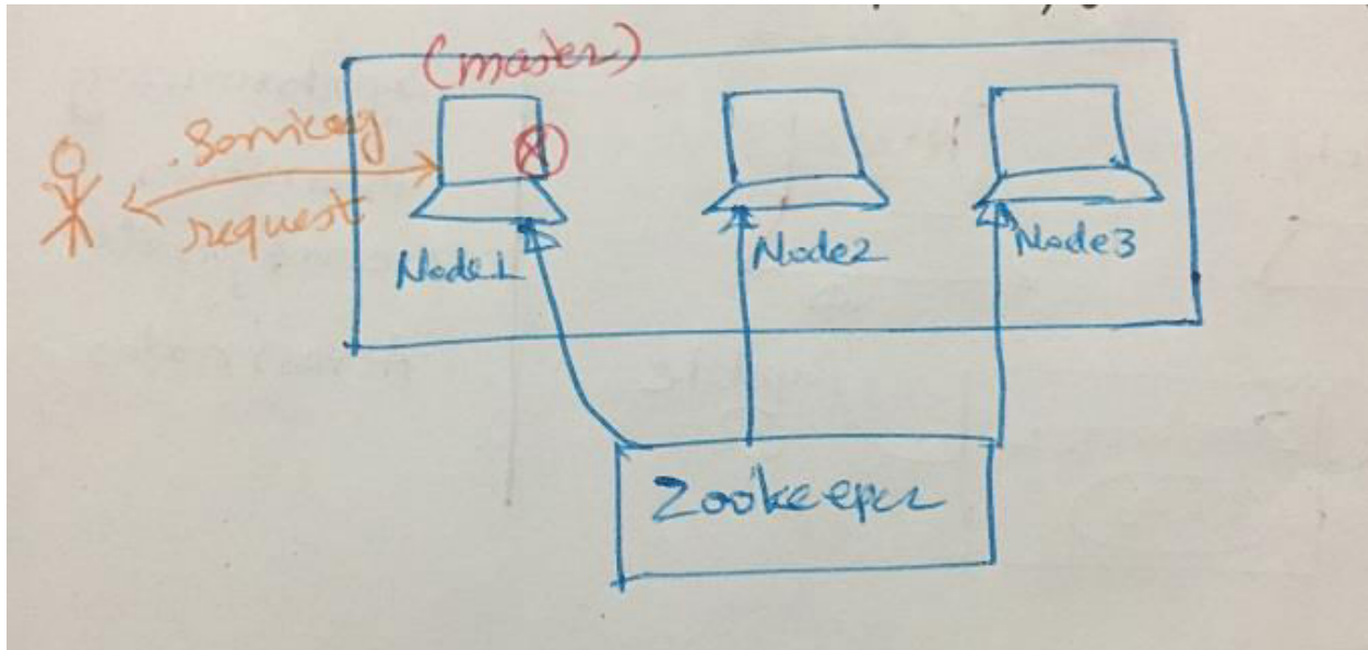
Hadoop NameNode: Active and StandBy namenode co-ordination
